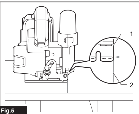
Fig.5 ► 1. Side edge of the base 2. Cutting line
