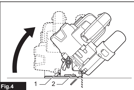
Fig.4 ► 1. Clamping screw 2. Bevel scale plate
